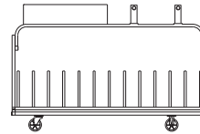
RT Cart—Edge 60 holds (10) RT 1860, 2460, 3060 tables 72 holds (20) 3636 or (10) RT 1872, 2472, 3072, 3672 tables 96 holds (10) RT 1896, 2496, 3096, 3696 tables PART #: CRT18-60EBLK2
